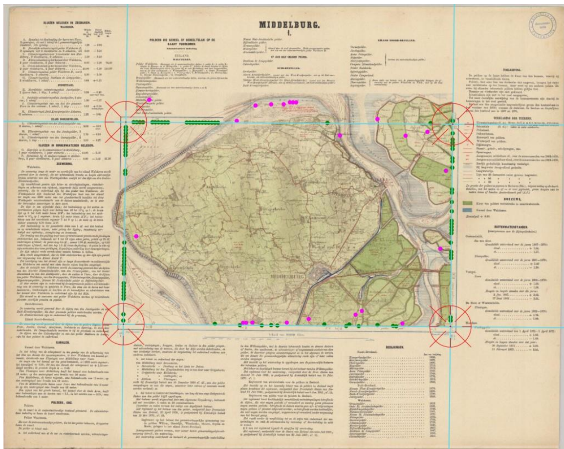
Figure 9: A processed sheet (Middelburg 1) of the Dutch historic water management map. In dark green the points found along the rim, which were accepted as inliers. The pink points are considered outliers. In blue the fitted lines with the RANSAC algorithm. The red crop marks indicate the intersection points of the lines, forming the GCPs in image coordinates and the corners of the polygonal mask for the sheet. Note, a neat line is partially absent around the top right corner.
